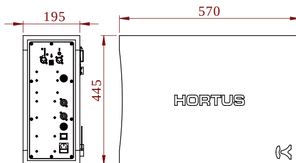
Dimensions version passive
