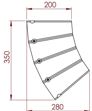
EU-13991 Tube ø35 mm & M20
